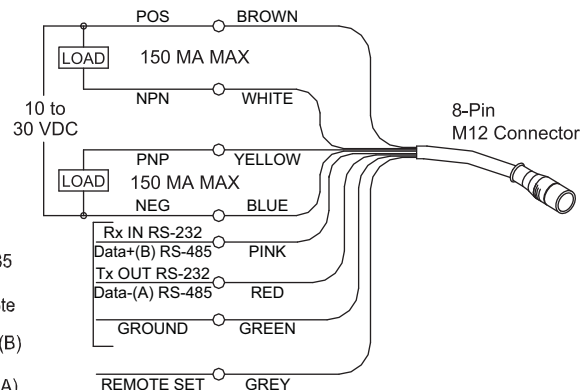
WIRING XPC4 (RS-485)
