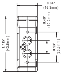
P/N SEB-3 Optional Mounting Bracket With Hardware
