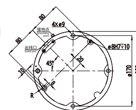
FR16 Pedestal diagram
