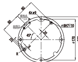
FR10 Pedestal diagram
