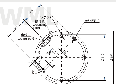
FR3-WML Pedestal diagram
