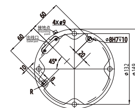
FR5 Pedestal diagram
