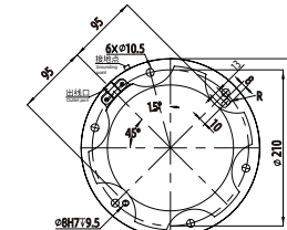
FR20 Pedestal diagram
