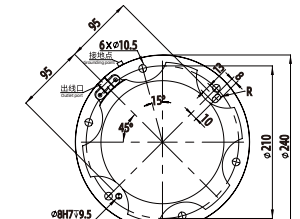
FR30 Pedestal diagram
